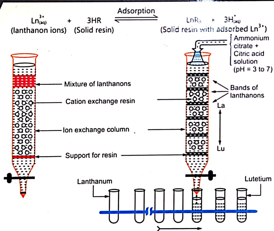
Separation of Lanthanons by Ion Exchange Chromatography
